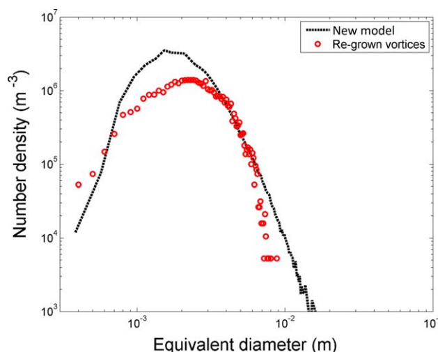
Figure 6. Number density distribution of turbulent vortices (regrown vortices) quantified using the vortex-tracking algorithm.
